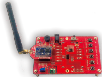
LoRa Demo Board
